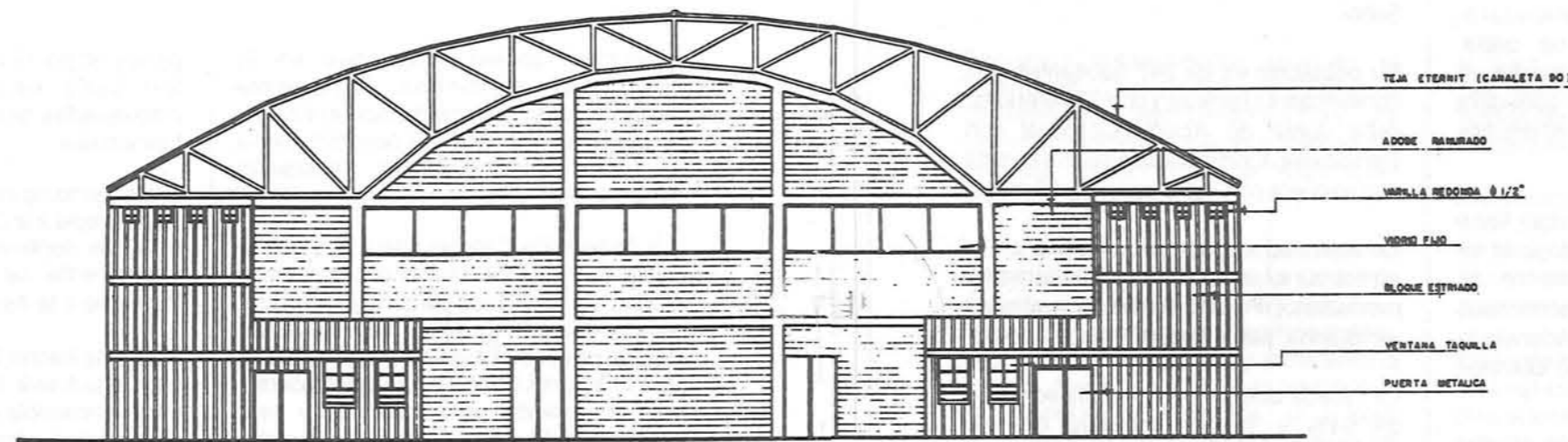
FACHADA PRINCIPAL
